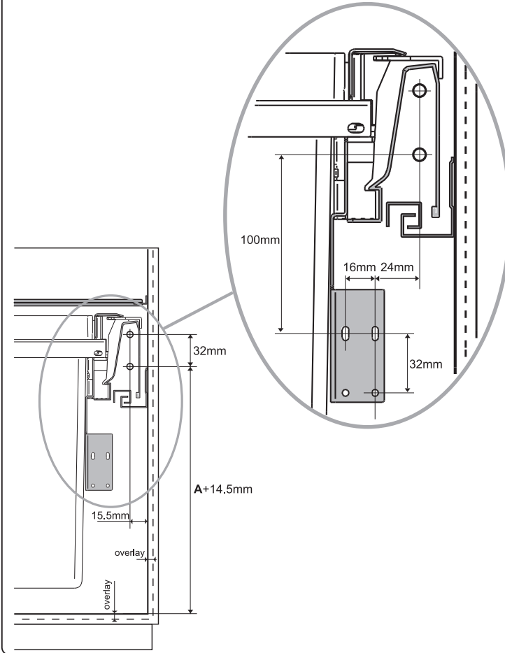
Blum Tandembox drawer front drilling position
