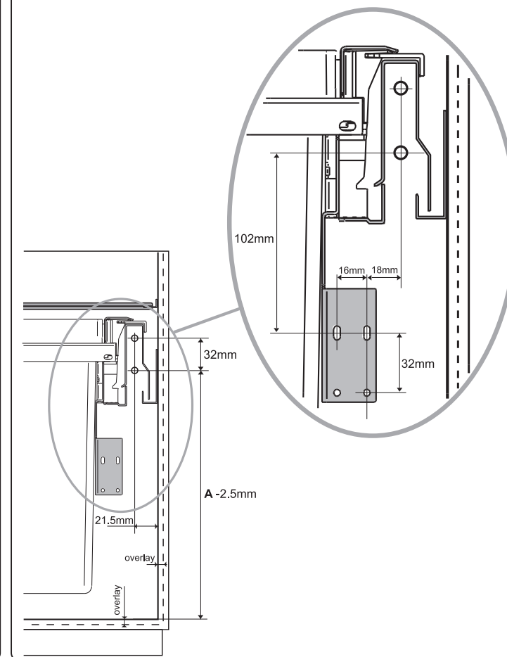
Grass Nova Pro drawer front drilling position
